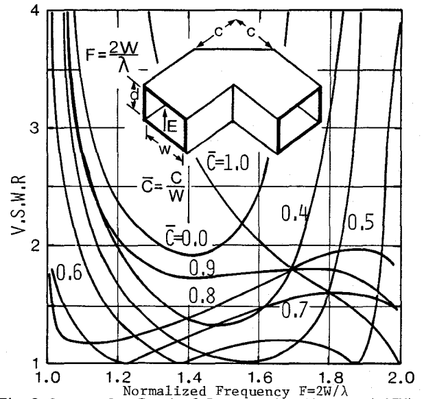
Fig.9 Corner-Cut Bend of Rectangular Waveguide(TM)
