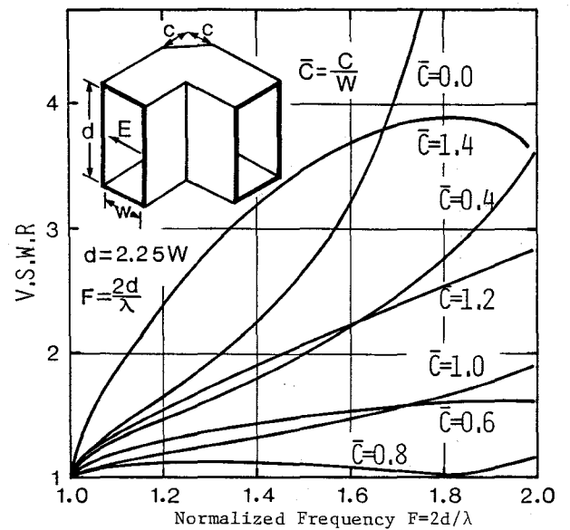
Fig.10 Corner-Cut Bend of Rectangular Waveguide(TE)
