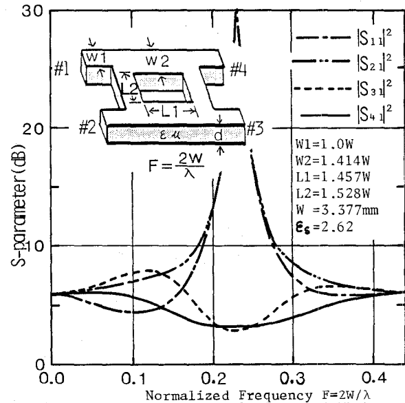
Fig.5 3-dB Hybrid Strip Line (TM)
