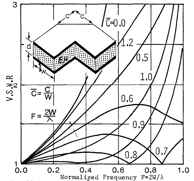
Fig.11 Corner-Cut 90° Bend of Strip Line(TM)
