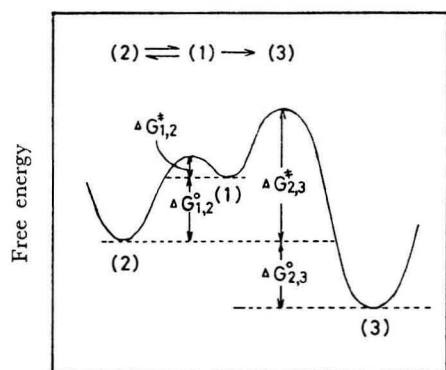
Fig. 3. Energy diagram between 1 , 2 , and 3 .
