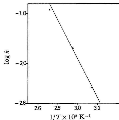
Fig. 2. Arrhenius plot,
